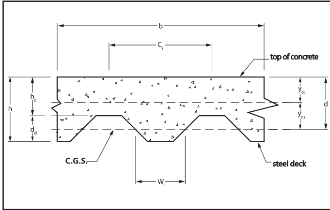
Figure C5.1-Composite Section
