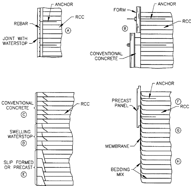
Fig. 5.5—Upstream facing options.
