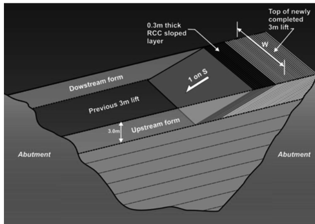
Fig. 6.10—Sloped layer placing method (SLM) (Forbes 1999).
