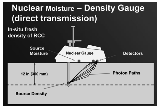
Fig. 7.3—Single-probe nuclear gauge. (Photo courtesy of Troxler Electronic Laboratories, 1981.)
