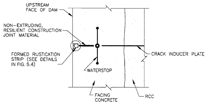
Fig. 5.3—Contraction joint detail.
