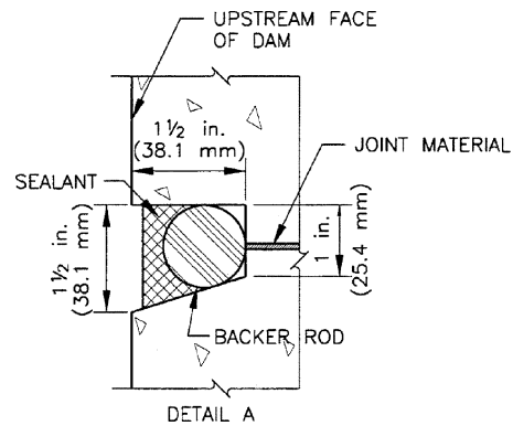
Fig. 5.4—Contraction joint seal at upstream face.
