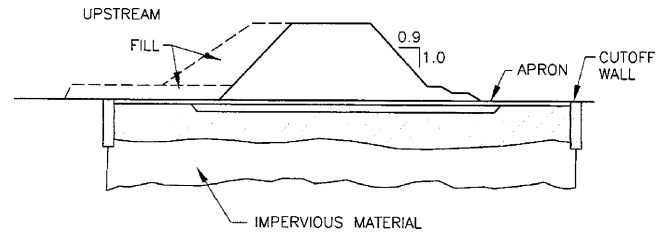
Fig. 5.2—Typical low RCC dam section for nonrock foundation.
