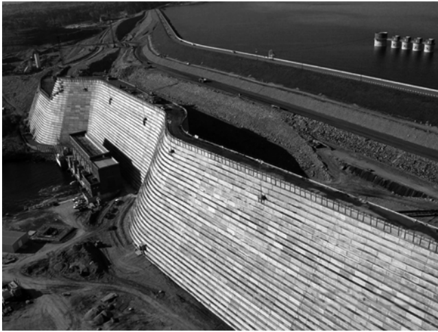
Fig. 6.18—Precast concrete forms for vertical upstream and stair-step downstream faces of Slauda Replacement Dam, SC. (Photo courtesy of Barnard Construction, 2005.)
