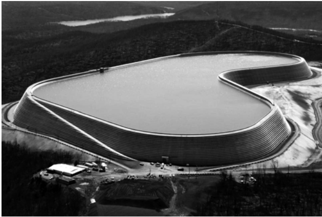
Fig. 1.5—Taum Sauk Dam, MO. (Photo Courtesy of ASI Constructors, Inc., 2007).
