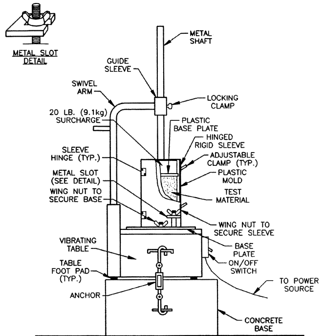
Fig. 7.4—Device for making RCC test cylinders with modified Vebe apparatus.
