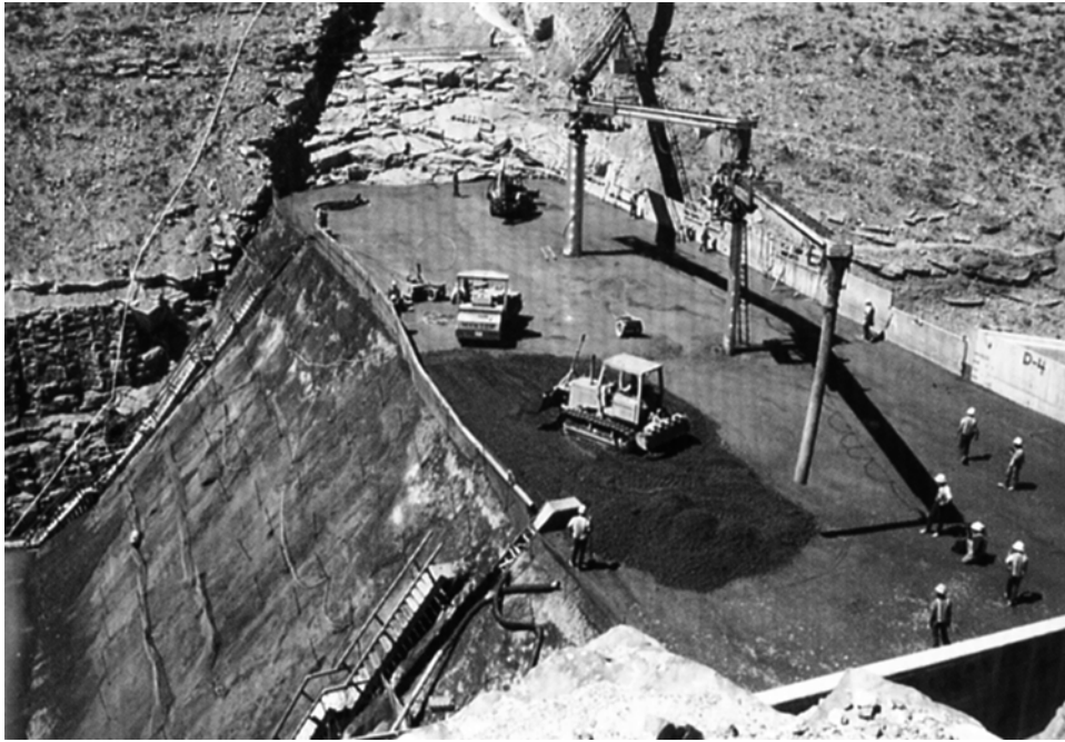
Fig. 6.4—All-conveyor RCC placing with embedded steel columns and “swinger” conveyor.
