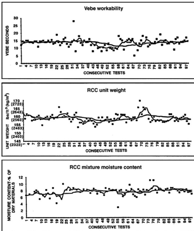
Fig. 7.7—Typical control charts for consecutive testing of Vebe, unit weight, and moisture content.
