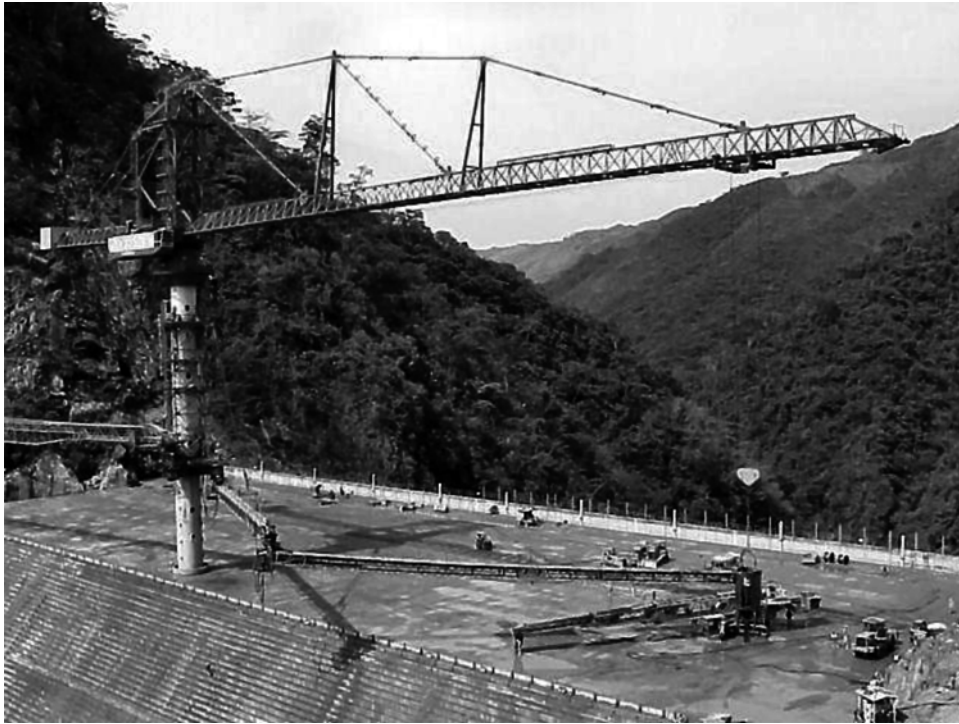
Fig. 6.6—All-conveyor RCC placing system for Miel I Dam, Colombia. (Photo courtesy of INGETEC S.A., 2002.)
