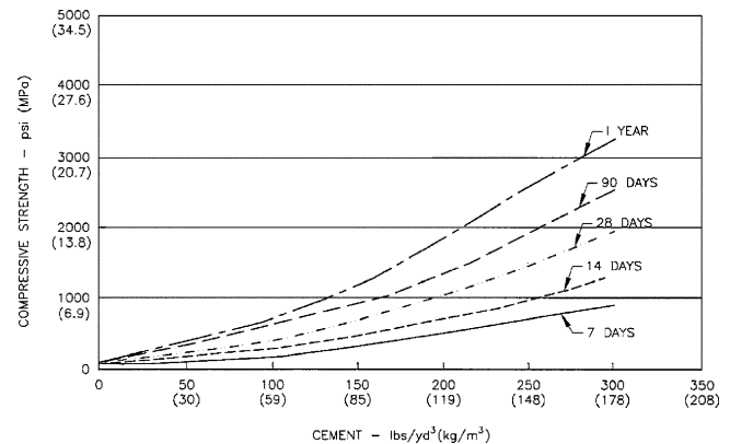
Fig. 4.2—RCC strength curves developed for lesser-quality aggregates.
