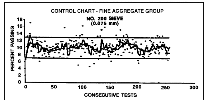
Fig. 7.6—Typical control charts for tracking fine aggregate grading results by selected individual sieves.
