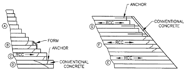
Fig. 5.6—Downstream facing options.
