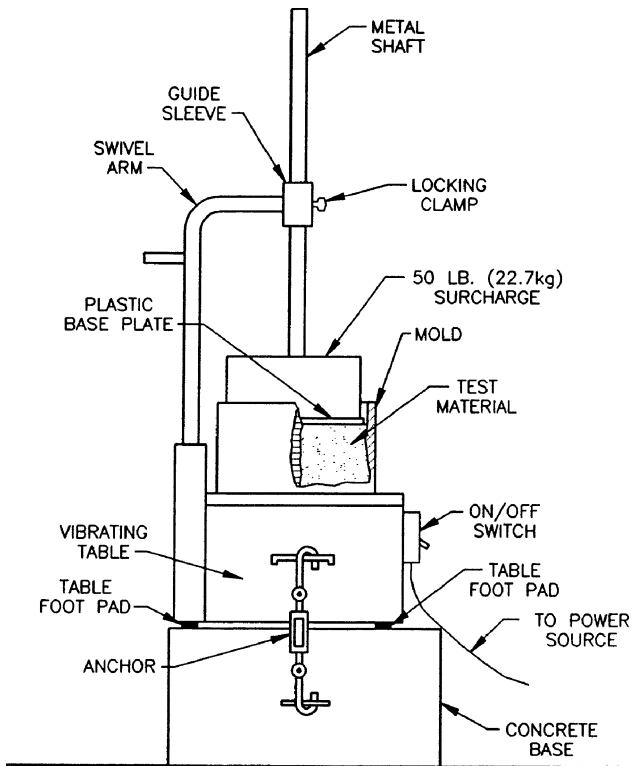
Fig. 7.1—Vebe consistency apparatus (ASTM C1170).
