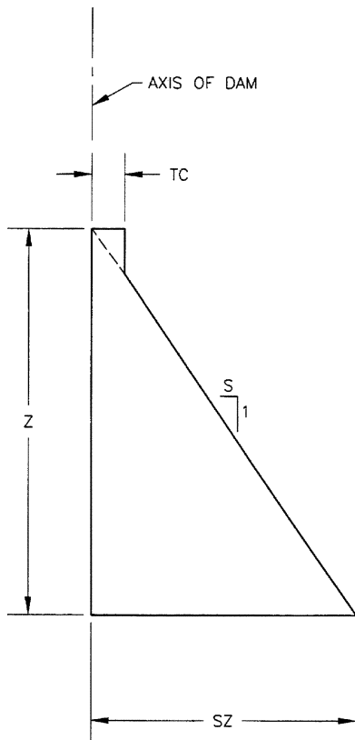
Fig. 5.1—Typical RCC dam section.
