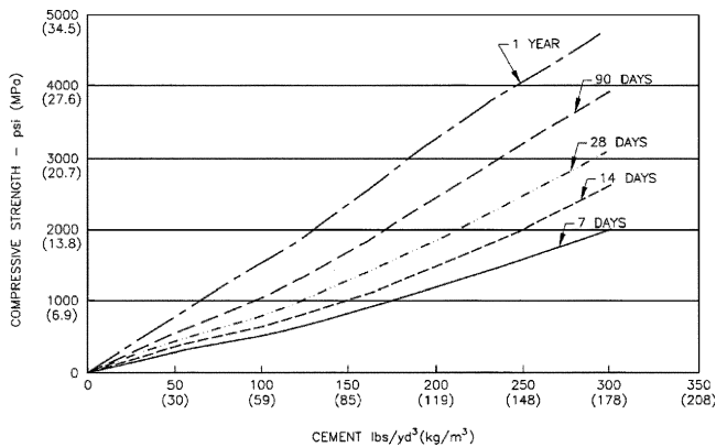
Fig. 4.1—RCC strength curves that can be developed from tests conducted on concretes with varying proportions of cement for high-quality aggregates.
