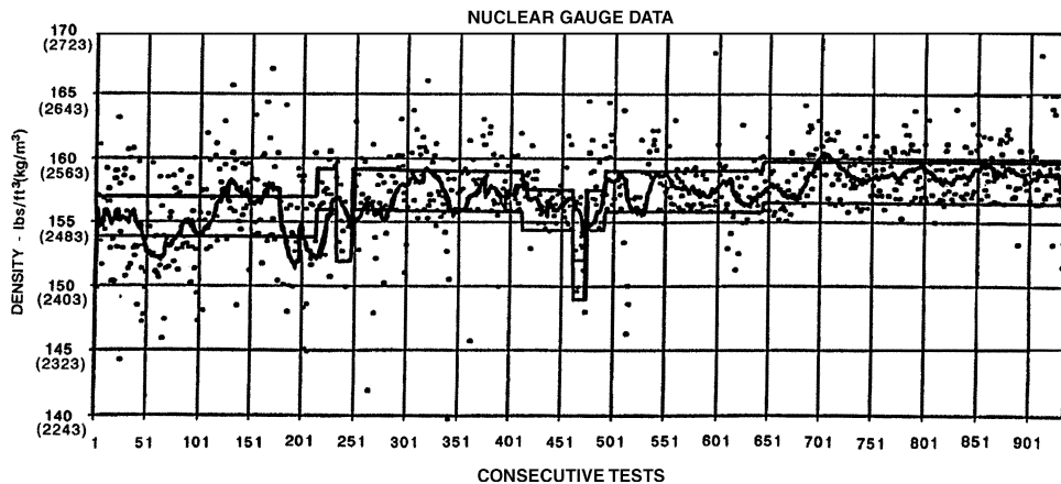
Fig. 7.8—Typical control chart for consecutive wet density test results.
