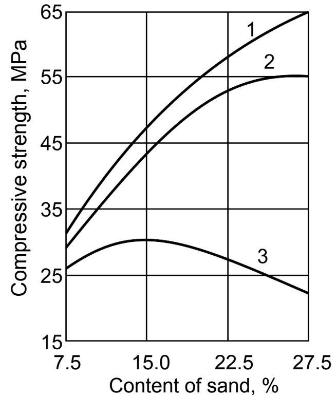
Fig. 10.2. Relationship between silicate concrete strength and sand content with specific surface:
