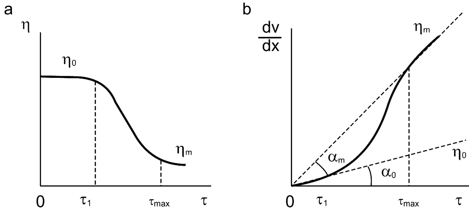
Fig. 2.1. Change of viscidly-plastic properties of concrete mixture depending on tensions:
