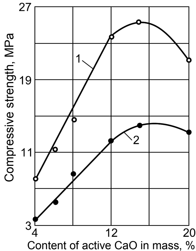
Fig. 10.1. Effect of active CaO in the mixture on compressive strength of lime-sand specimens:
