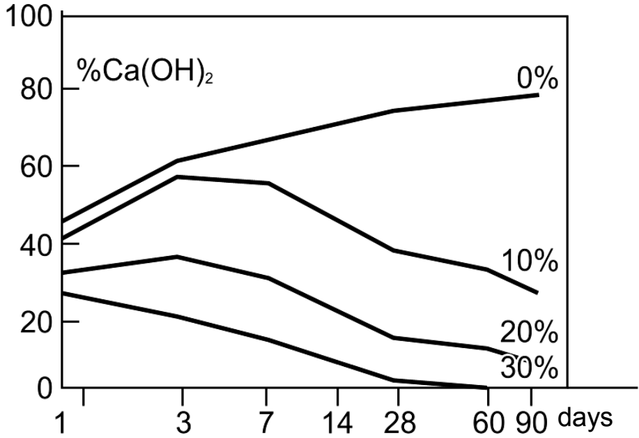
Fig.3.13. Change of the quantity of calcium hydroxide Ca(OH) 2 in solutions containing metakaoline (finely divided product that results from burning of kaolin)
