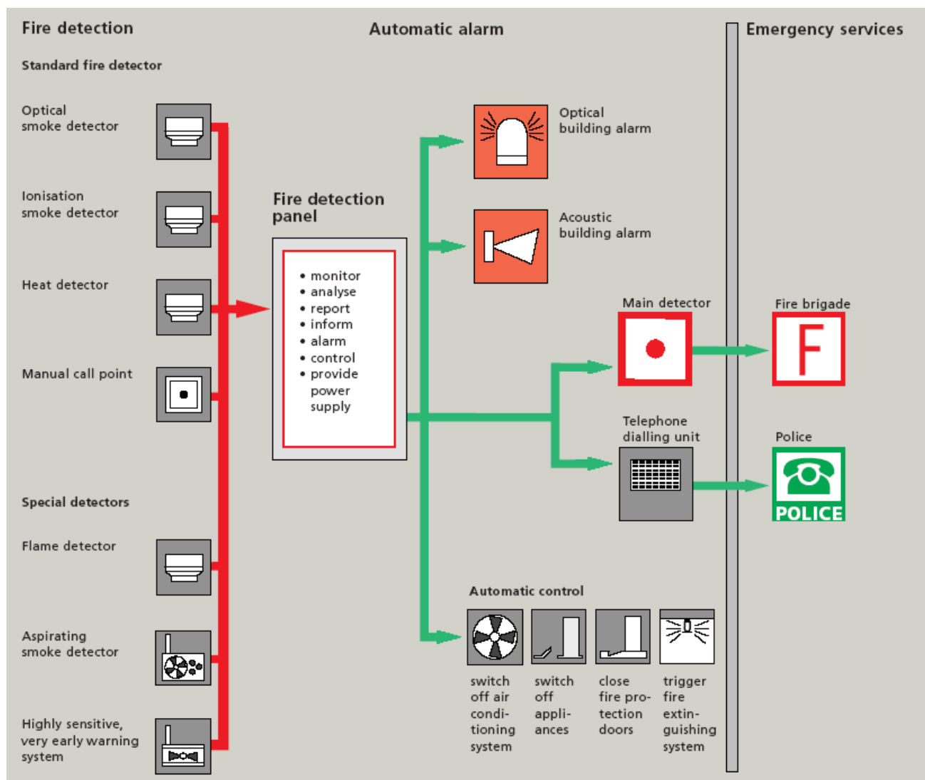
Logic diagram of a Minimax fire detection system
