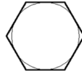
Circumscribed about circle
